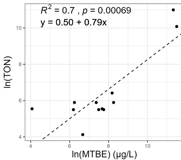
Figure 13. Scatter plot of threshold odour number (TON) vs MTBE on a logarithmic scale and regression equation, where y = \ln(\text{TON}) , x = \ln(\text{MTBE})
