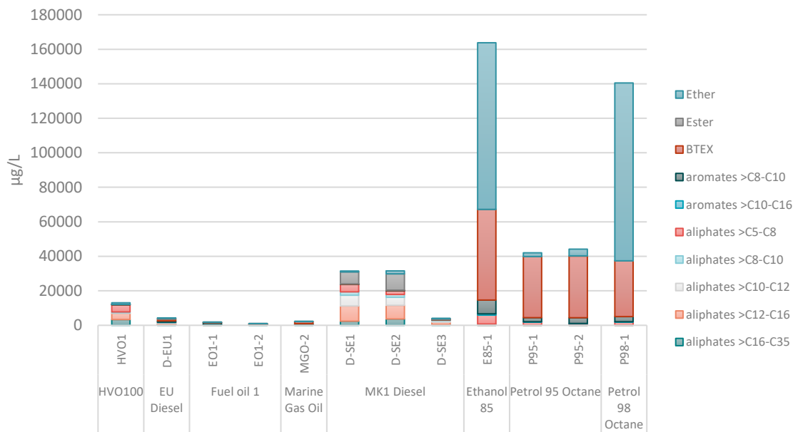
Figure 7. Total concentrations of the determined substances in the WAF per SPIMFAB substance group. Note that sums of substance groups only contain the quantified substances in this study and not the sum of the entire substance group.
