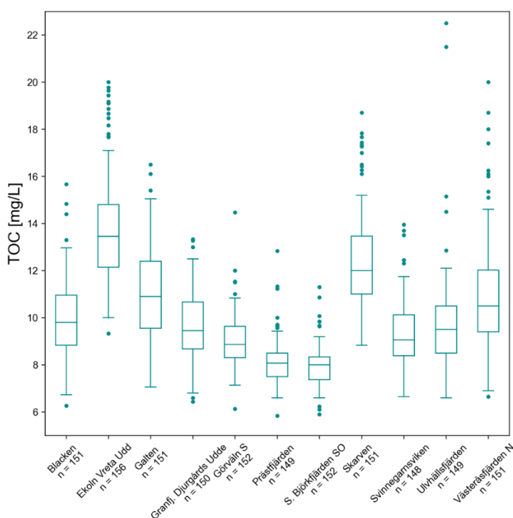
Figure 22. Box and whisker plot of concentrations (mg/L) of n total organic carbon (TOC) data from the Swedish environmental monitoring retrieved from the Miljödata-MVM database. The values are average concentrations of field replicates, if available.
