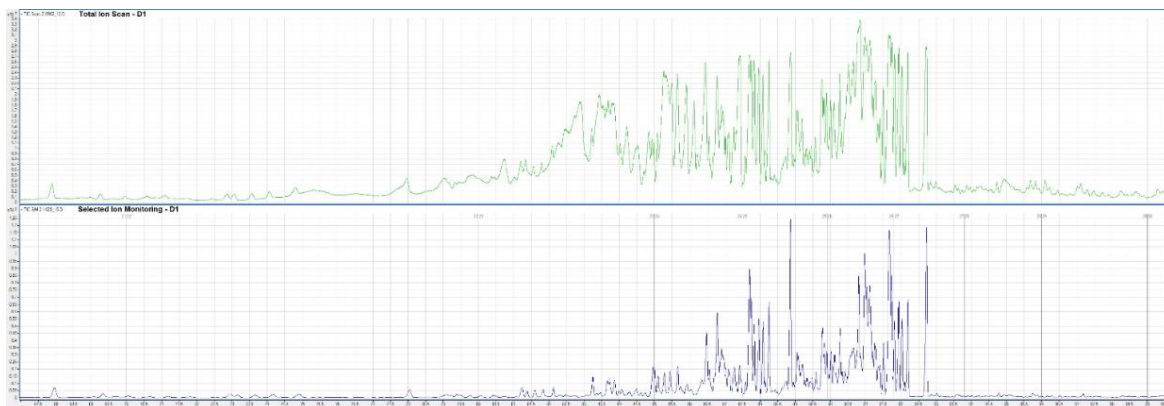
Figure 6. GC/MS chromatograms of HVO-1 fuel in full scan (upper) and Selected Ion Monitoring (lower).
