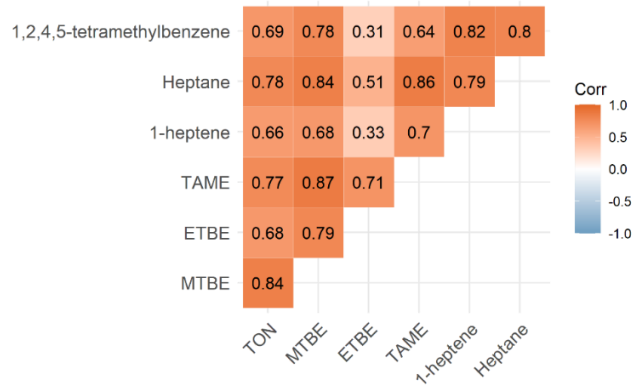
Figure 12. Correlation matrix for selected substances with TON. Natural logarithm was applied to all data before calculating correlations.
