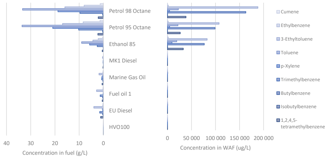
Figure 8. Concentrations of selected aromatic compounds in the fuels, right, and in the WAF, left.
