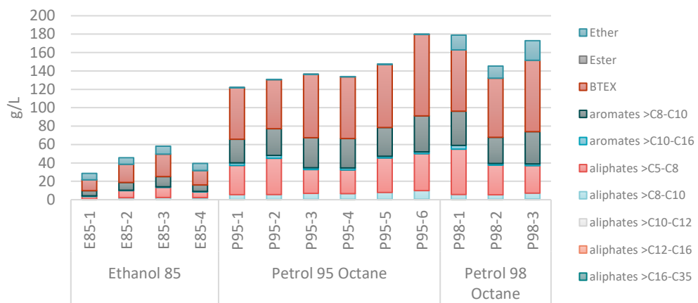
Figure 3. The sum of analysed substances per SPIMFAB group in petrol and petrol-like fuel. Note that sums of substance groups only contain the quantified substances in this study and not the sum of the entire substance group.
