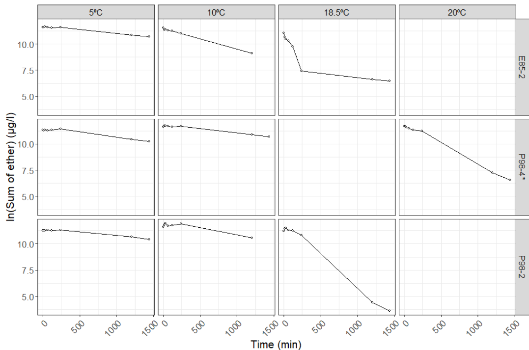
Figure 19. Plots of the sum of ether on a logarithmic scale vs time for the aeration test. Plots are separated by the temperature of the test and by fuel.
