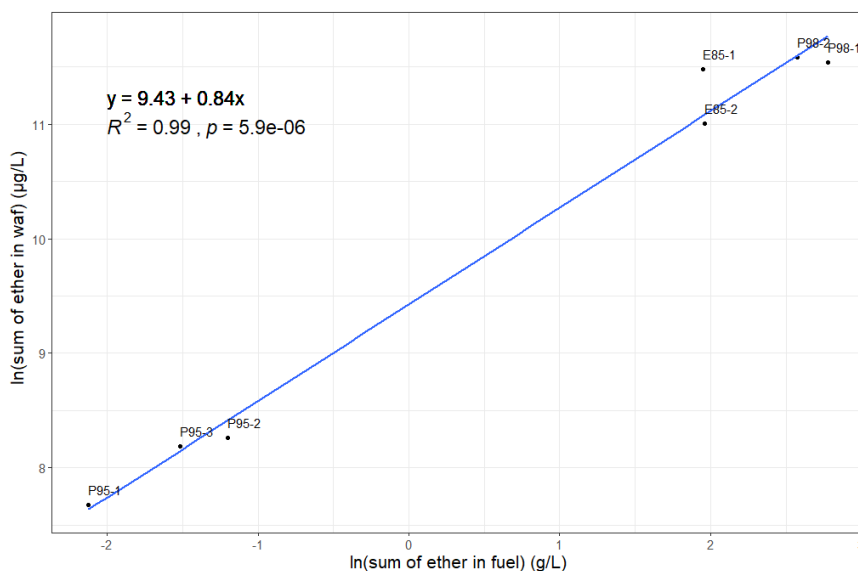
Figure 10. Scatter plot of the sum of ether in WAF vs in fuel on a logarithmic scale and regression equation, where y = \ln(\text{sum ether in WAF}) , x = \ln(\text{sum ether in fuel}) .
