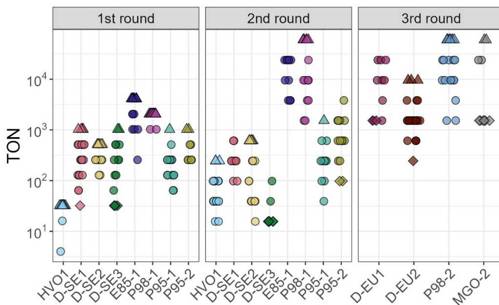
Figure 11. The threshold odour number, on a logarithmic scale, indicates where an odour first was noticed by each panel member. Triangles indicate a panel member noticing an odour in the most diluted sample, and diamonds indicate no odour in the least diluted sample. Dots indicate a panel member noticing an odour in any other bottle. In the 1 st round, a dilution factor of 2 was used, and in the 2 nd and the 3 rd round, a dilution factor of 2.5 was used. One colour per fuel type for better visual separation.
