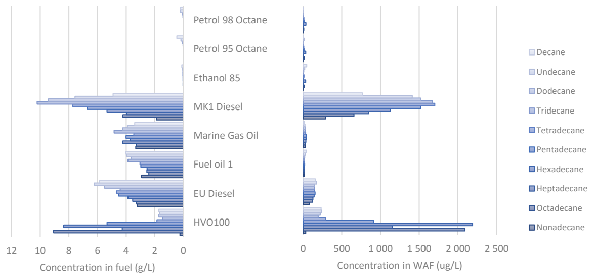
Figure 9. Concentrations of selected aliphatic compounds in fuels and in WAF.
