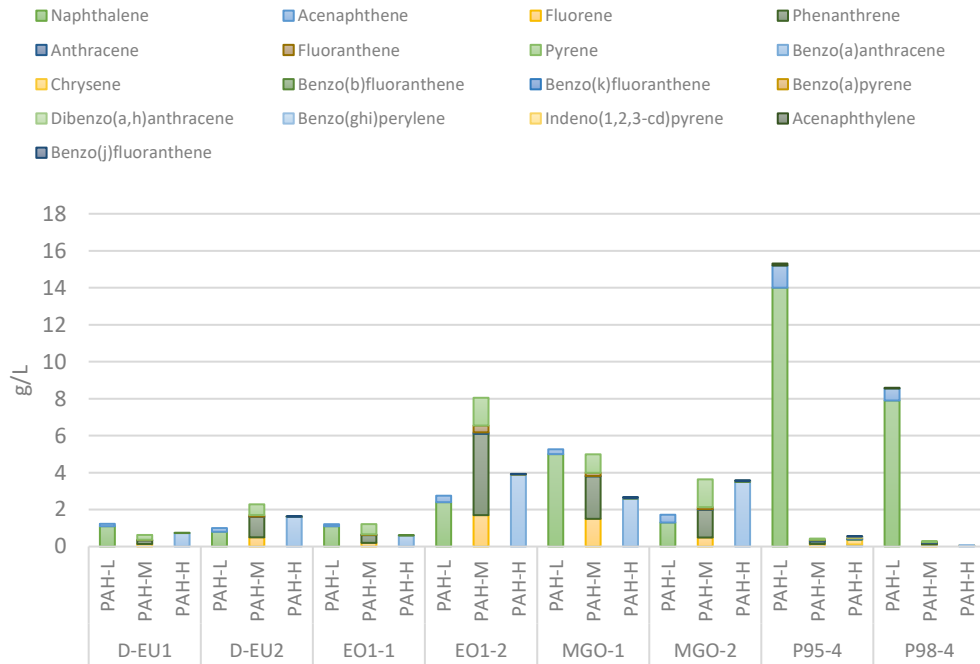
Figure 5. Concentrations of PAH compounds in eight fuel samples grouped in PAH-L (low molecular weight), PAH-M (medium molecular weight) and PAH-H (high molecular weight). The definition is found in annex 2.
