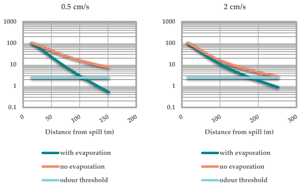
Figure 3 Concentration of ether as a function of the distance from the spill in meters.
