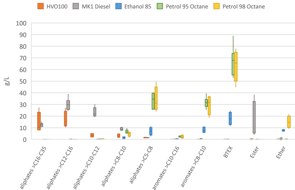
Figure 4. Box and whisker plot of concentrations (g/L) of SPIMFAB compound groups in the study with three or more samples in fuel products. Note that sums of substance groups only contain the quantified substances in this study and not the sum of the entire substance group. The plot features boxes that represent the interquartile range (IQR), extending from the first quartile (Q1) to the third quartile (Q3) and enclosing the median, marked by a line within each box. Whiskers extend from the boxes to the furthest data points within 1.5 times the IQR, capturing the overall range of the data while excluding outliers.
