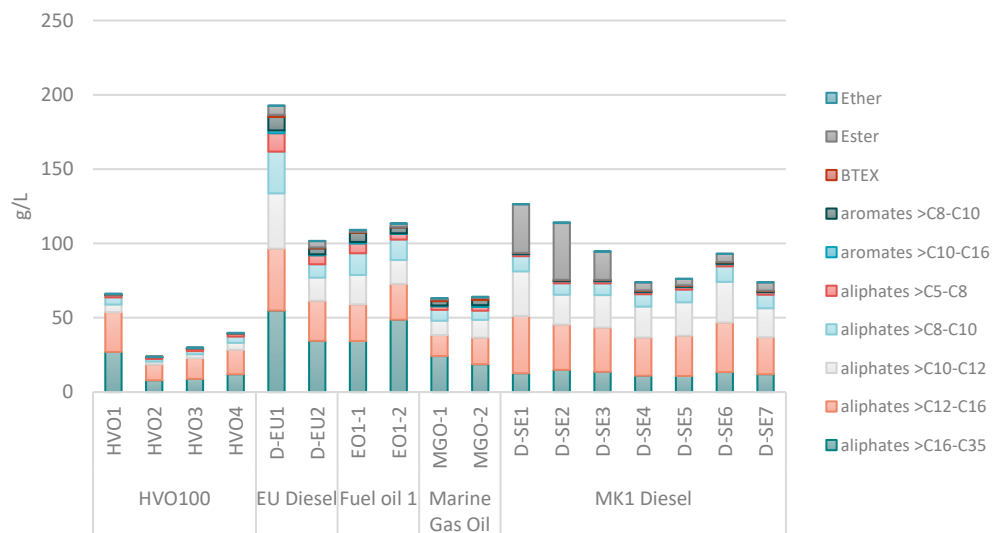
Figure 2. Total concentrations of the SPIMFAB substance groups in diesel and diesel-like fuels. Note that sums of substance groups only contain the quantified substances in this study and not the sum of the entire substance group.
