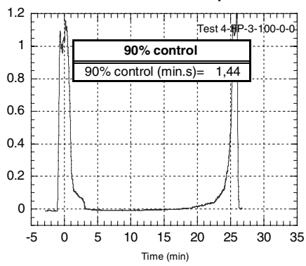
Relative radiation FFFP-AR 3% Heptan
