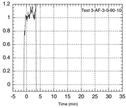
Relative radiation AFFF-AR 3% Bensin+10% etanol
