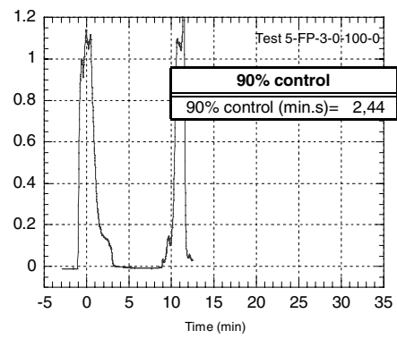
Relative radiation FFFP-AR 3% Bensin
