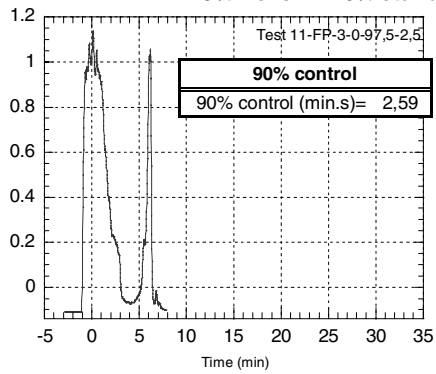
Relative radiation FFFP-AR 3% Bensin+2.5% etanol
