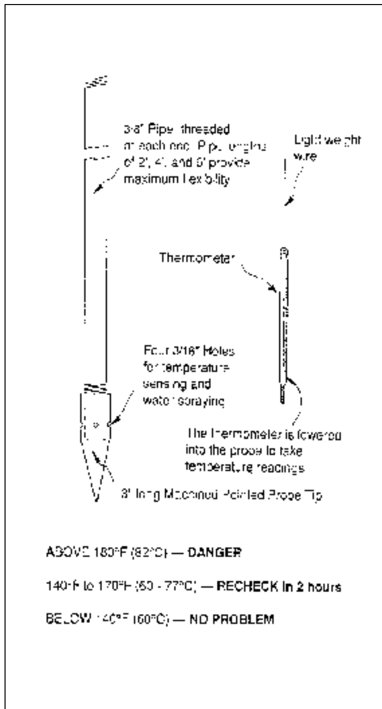
Diagram 9. Temperature Probe
