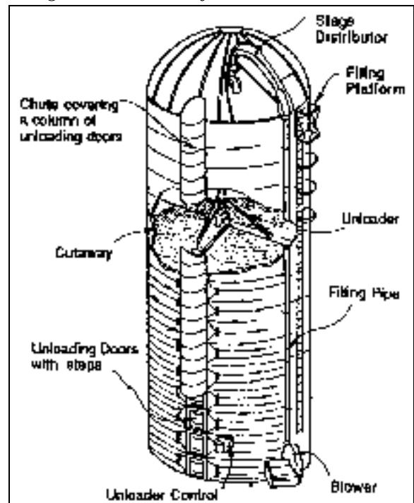
Diagram 2. Features of Conventional Vertical
