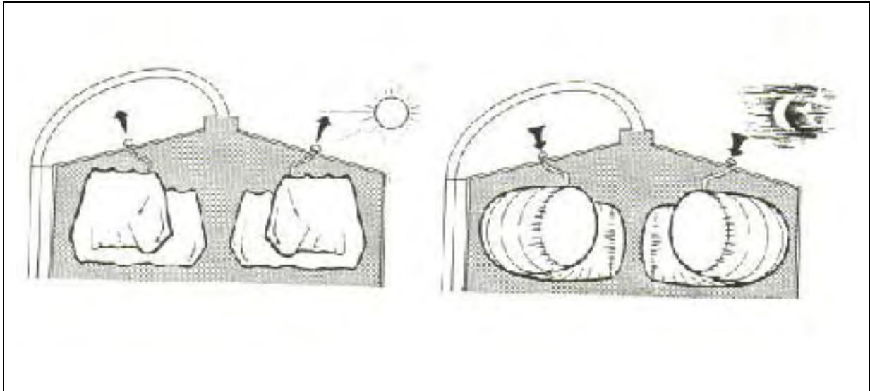
Diagram 6. “Breather Bag” system in oxygen-limited silo
